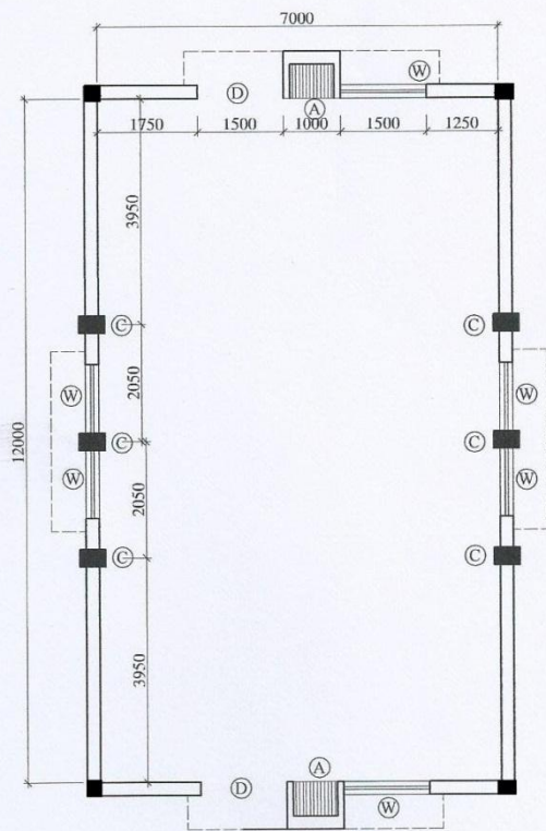
PLAN
