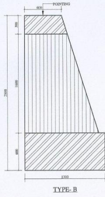
TYPE-B
